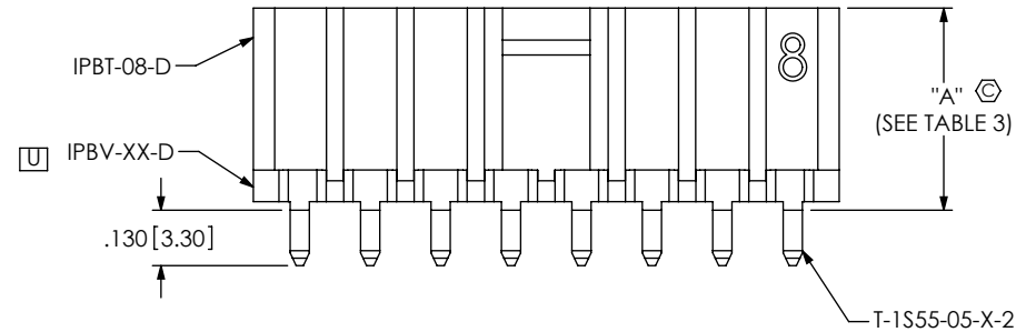
FIG. 5 (IPBT-108-H3-XX-D SHOWN) (DIFFERENT AS SHOWN, OTHERWISE SAME AS FIG. 1)
